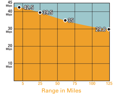
Performance with 5.8 and 5.4 GHz Connectorized Lite Models
