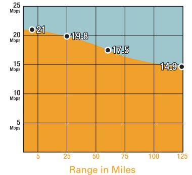
Performance with 5.8 and 5.4 GHz Connectorized Lite Models
